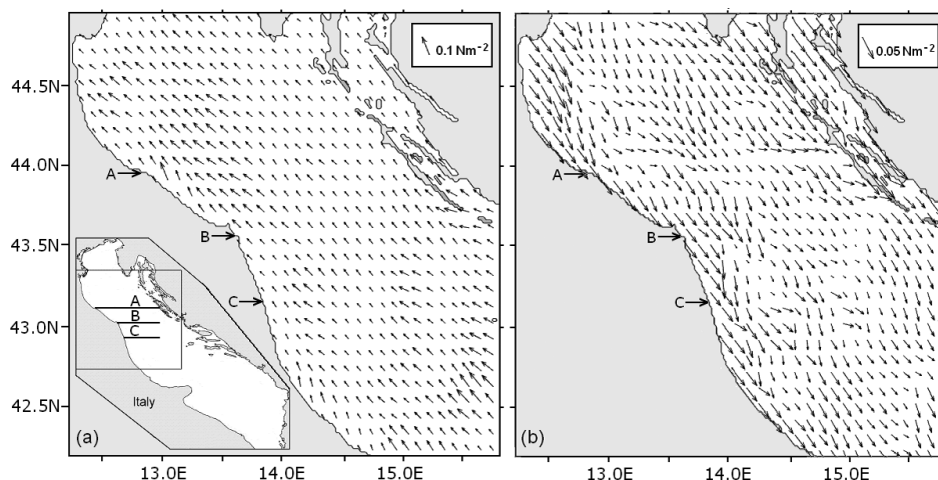
Figure 1. Patterns of Sirocco (a) and Mistral COAMPS (b) winds over the northern and central Adriatic. The three straight lines across the Adriatic basin shown in the frame and labeled by A, B and C indicate transects for the simulations of current velocity and density. In the panel, arrows A, B, and C denote initial points of each transect.
