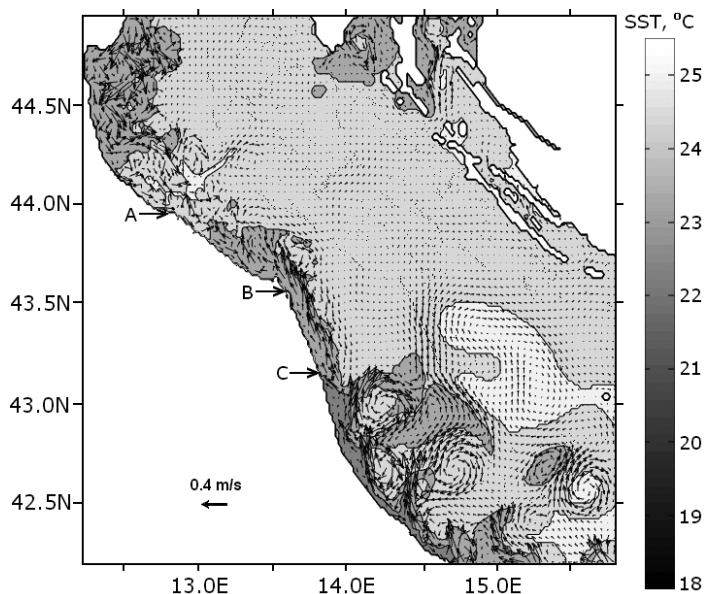
Figure 3. Daily averaged SST and SSV (for July 12, 2003) at the beginning of the development of upwelling zones and the WAC reversal along the Italian coast under the combination of steadily blowing Sirocco winds (see Figures 1a) and a low Po River discharge rate.
