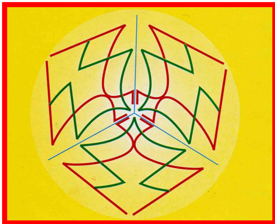
Mathematical rose
