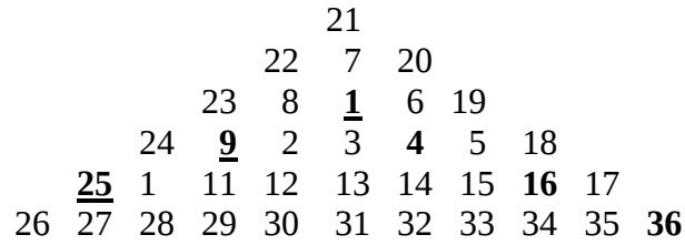
Fig. 5 Triangular spiral. \{A_n\} = \{n\}
